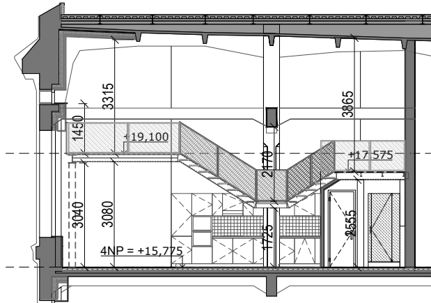
REZ
